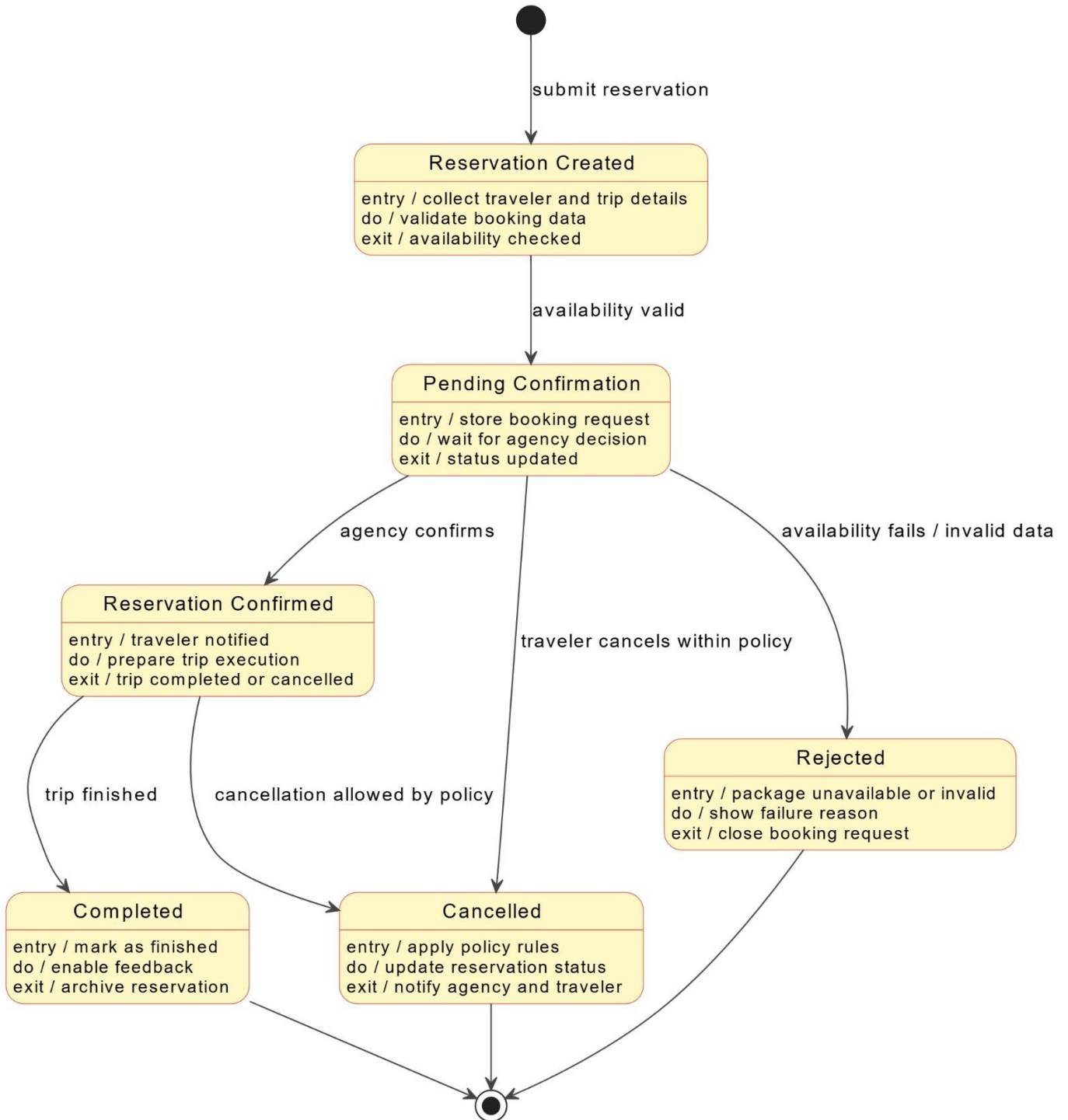
Booking / Reservation State Diagram
